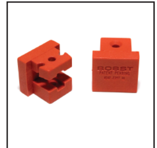
Centering Block BSA 0502 2397 00 BSA 0502 2094 00
